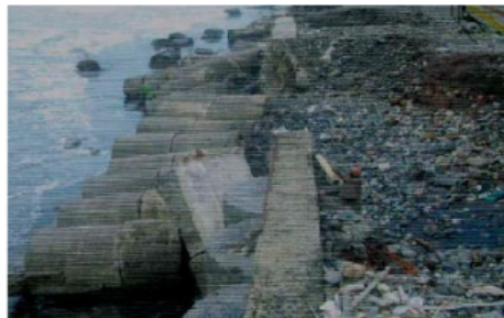
Figure2. The damageson the seawall south Pasauran beach (Junarsa, 2006)
